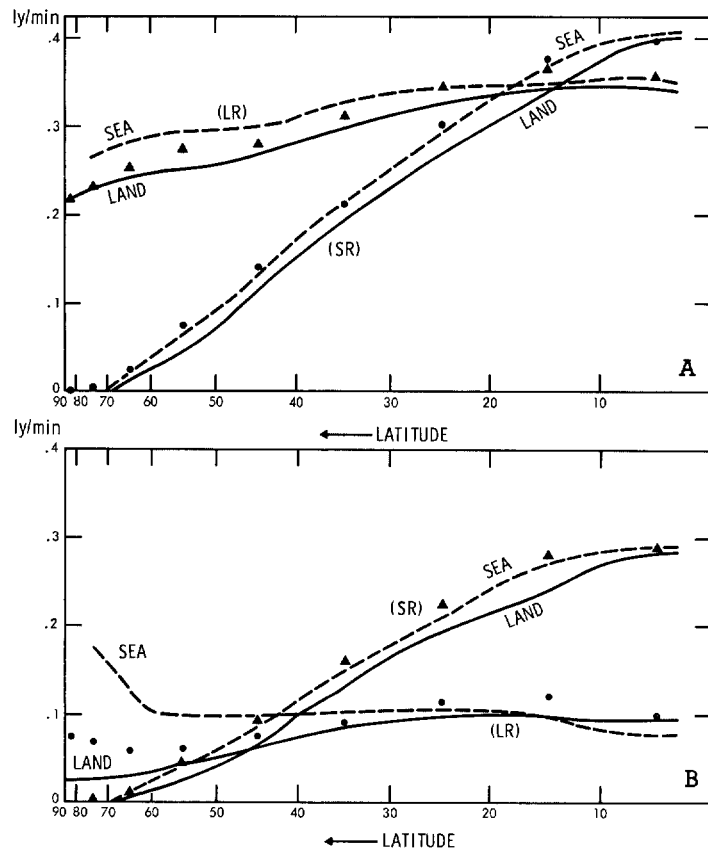
FIGURE 43.—The computed radiation averaged for 14 days in Experiment 2 for the 1964 case. (SR) is the net downward solar radiation, and (LR) the net upward longwave radiation. The quantities over land (solid lines) and over sea (dashed lines) are shown. The dotted curves (small solid circles and triangles) are SR and LR for winter by London (1957), with no distinction between land and sea. Figure (A) is at the top of the atmosphere, and (B) is at the earth's surface.
