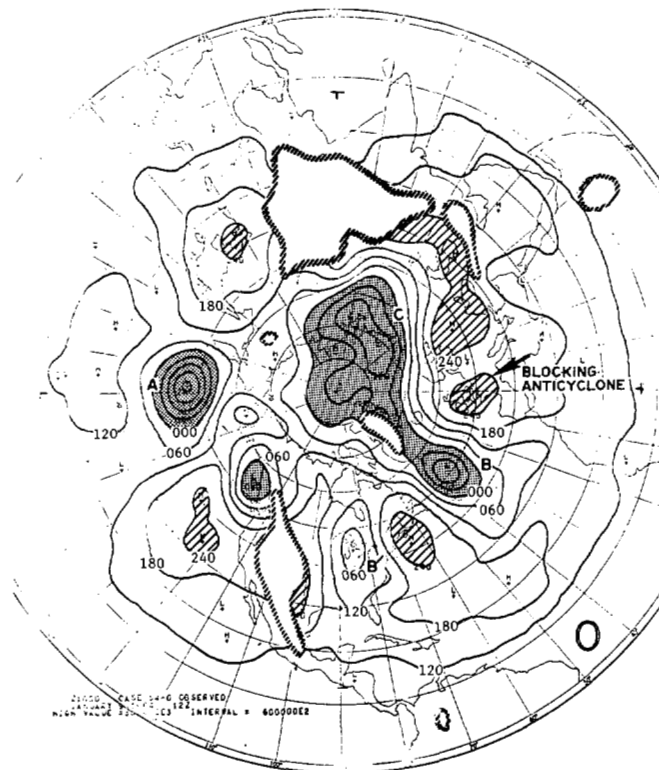
FIGURE 49.—The observed (0 day and left columns) and Experiment 3 (right columns) 1000-mb geopotential height patterns for the period 0 to 14 days commencing at 1200 GMT, Jan. 9, 1964. The contour interval is 60 m. The anticyclone areas with the geopotential value greater than 240 m are hatched, and the cyclone areas with the geopotential value less than 0 m are stippled. The mountains are blank areas enclosed by small segmented lines. The number in the lower right corner is the day of the forecast. “Blocking anticyclones” and “newly formed cyclones” are indicated by the respective letters and arrows. The letters A, B, C, etc. are used for identification.
