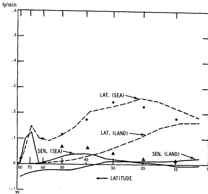
FIGURE 18.—Latitudinal distribution of turbulent heat flux at the lower boundary in Experiment 3, averaged for 10 days. See figure 9 for further explanation.
