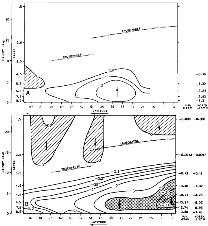
FIGURE 84.—Vertical flux of water vapor by eddies \left(\frac{p \cdot \bar{\omega}}{g}\right) \cdot r' in units of 10^{-7} \text{ gm cm}^{-2} \text{ sec}^{-1} . (A) from the \omega -equation, valid between 850 and 500 mb, and (B) the prediction. See figure 64.
