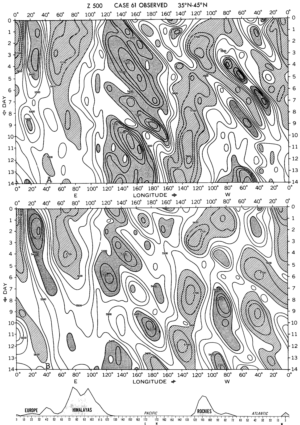
FIGURE 87.—Trough-and-ridge diagrams for 35°-45° lat. at 500 mb in the 1966 case. (A) the observed, and (B) the prediction. See figure 22.
