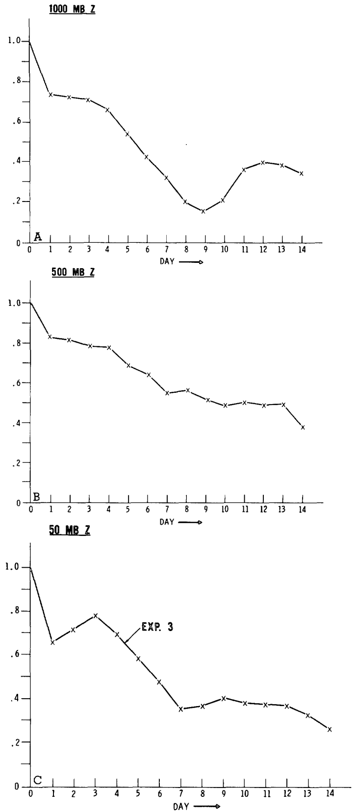
FIGURE 90.—Correlation coefficient for the observed and predicted patterns of time change of the geopotential heights for the 1966 case. (A) 1000 mb, (B) 500 mb, and (C) 50 mb. See section 7 and figure 25 for further details.
