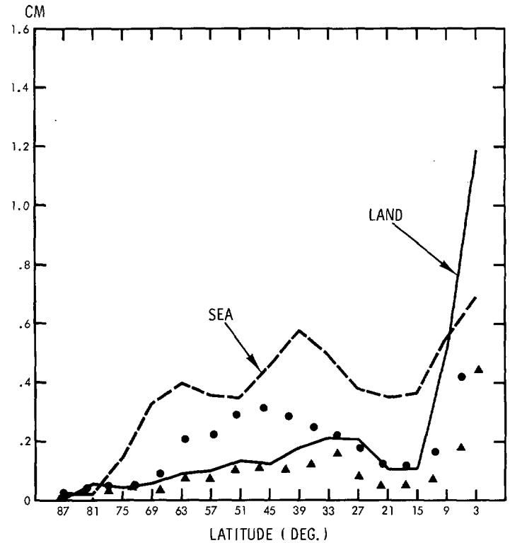
FIGURE 17.—Latitudinal distribution of the 24-hr rates of precipitation over land and sea in Experiment 3. See figure 8 for further explanation.
