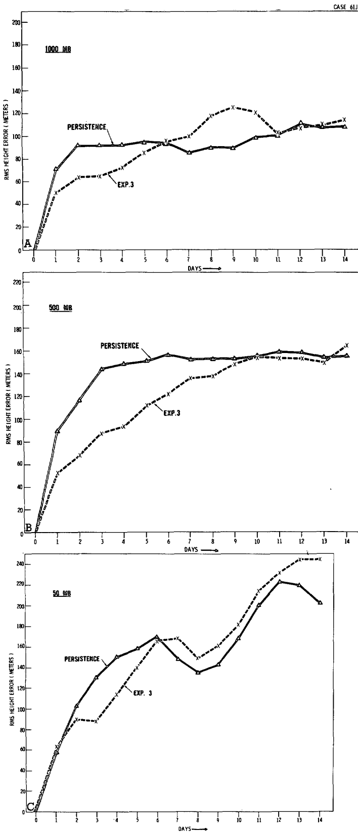
FIGURE 89.—Standard deviation of the difference between the observed and predicted geopotential heights for the 1966 case. (A) 1000 mb, (B) 500 mb, and (C) 50 mb. See section 7 and figure 24 for further details.
