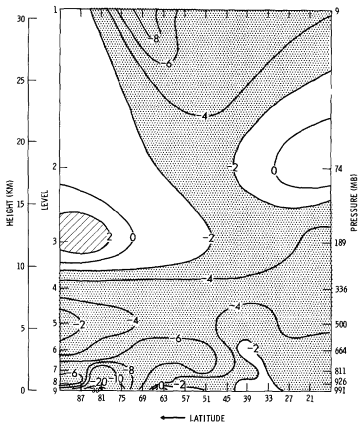
FIGURE 11.—Meridional section of the zonally averaged temperature error in Experiment 2 for the 11th day in units of ^{\circ}\text{C} . The areas where the difference is more negative than -2^{\circ}\text{C} are stippled, and those where the difference is larger than 2^{\circ}\text{C} are shaded. The ordinate is the vertical level.
