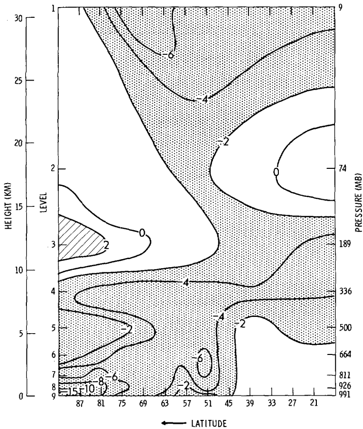
FIGURE 16.—Meridional section of zonally averaged temperature error for Experiment 3 at the 11th day in units of °C. See figure 11 for the details.
