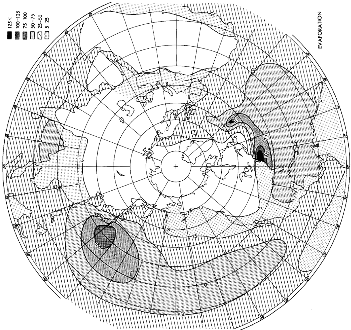
Figure 67.—Twenty-four-hour rate of evaporation in Experiment 3 of the 1964 case averaged for the period 3 to 14 days in units of 10^{-2} cm. In the polar region there are dry streaks which are the same phenomena as the so-called fictitious "land breeze" effect in figure 12. Comparing the computed evaporation for the 1964 (this figure) and 1966 (fig. 92) cases with Budyko's (1963) distribution (fig. 66), the following items are noted. 1) The computed distributions are more similar to each other than to Budyko's distribution. 2) In his map, there are three major evaporation regions in the Northern Hemisphere, i.e., the Gulf Stream , the Kuroshio Current , and the North Atlantic . In the computed results these have been to some extent obtained, but the computed evaporation east of the Asian Continent, i.e., near Japan, is smaller. 3) The computed evaporations near Mexico in the Pacific Ocean and over the Arabian Sea are very large. 4) The computed evaporation over land in the middle and low latitudes are large, especially over the Sahara Desert for instance.
