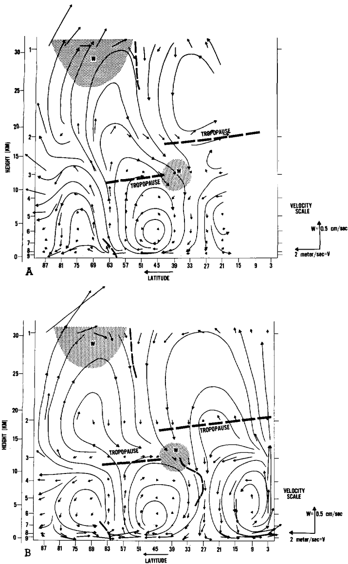
FIGURE 39.—Meridional circulation. The arrows plotted at the gridpoints are drawn according to the scales shown in the lowest right corner. The centers of the tropopause jet and polar-night jet are indicated by shading and by (W). (A) obtained by solving the \omega -equation (see fig. 38) and (B) Experiment 3 (time averaged for 3 to 14 days).
