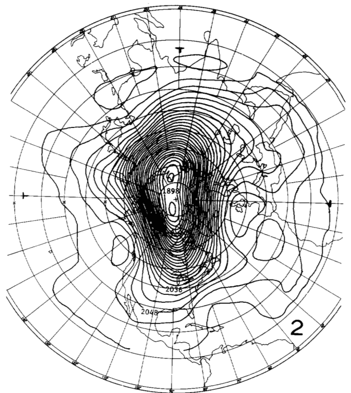
FIGURE 51.—The observed (left columns) and Experiment 3 (right columns) 50-mb geopotential height for 2 weeks commencing Jan. 9, 1964, in units of decameters. The contour interval is 60 m.
