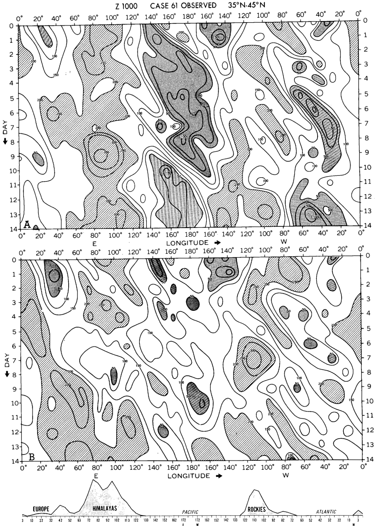
FIGURE 88.—Trough-and-ridge diagrams for 35°-45° lat. at 1000 mb in the 1966 case. (A) the observed, and (B) the prediction. See figure 23.
