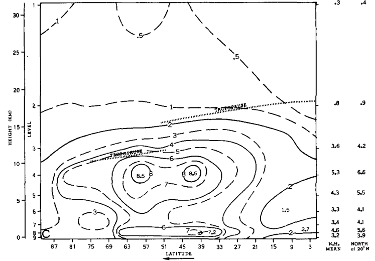
FIGURE 37.—Meridional section of the eddy kinetic energy \rho(\bar{u}^2 + \bar{v}^2)/2 in units of 10^3 ergs/cm 3 . The regions where the intensity is larger than 10^3 ergs/cm 3 are crosshatched. The maxima are plotted. (A) the observed (time averaged for the period 0 to 14 days), (B) Experiment 2, and (C) Experiment 3 (the latter two are averaged for 3 to 14 days).
