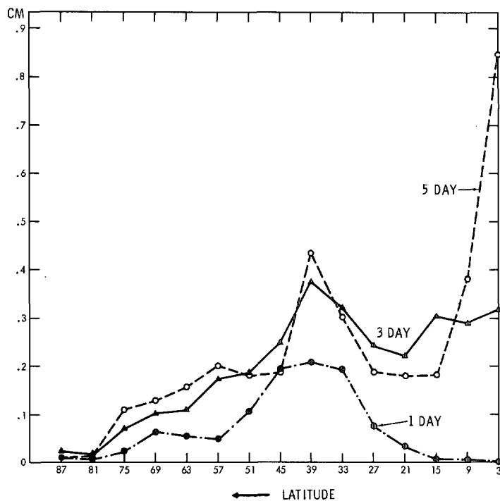
FIGURE 6.—Time variation of the latitudinal distribution of the 24-hr rate of precipitation in Experiment 2. The curves are for 1, 3, and 5 days.
