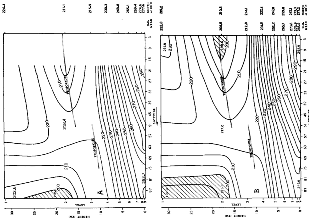
FIGURE 54.—Temperature \bar{T} in units of °K. (A) the observed, and (B) the prediction.
