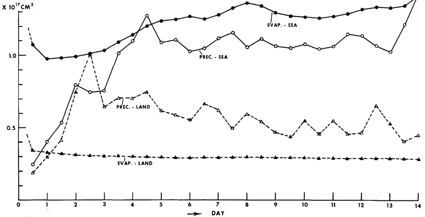
FIGURE 46.—The time variation of the 6-hr rates of precipitation and evaporation in Experiment 2. Both quantities are the total volumes over land and sea for the whole hemisphere. Note that the precipitation was maximum at 2.5 days over land.
