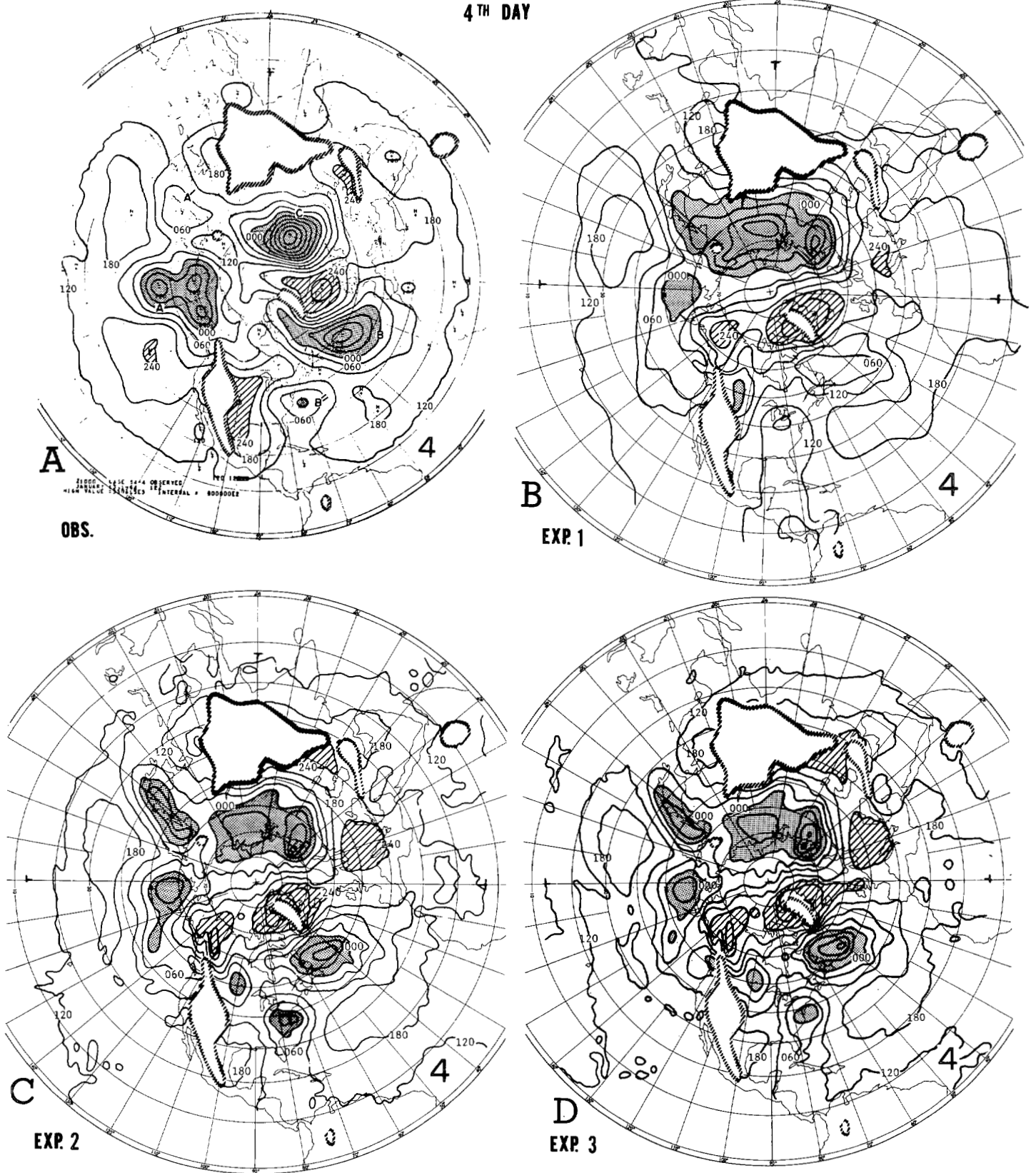
FIGURE 20.—The 1000-mb geopotential height for the 4th day. (A) the observed, (B) Experiment 1, (C) Experiment 2, and (D) Experiment 3.
