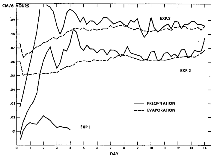
FIGURE 4.—Time evolution of the 6-hr rates of precipitation (solid lines) and evaporation (dashed lines) hemispherically averaged for Experiments 1, 2, and 3.
