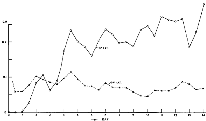
FIGURE 7.—Six-hour rates of precipitation at the two latitudes of maxima, 3° and 39°N, in Experiment 2. The abscissa is time in days.
