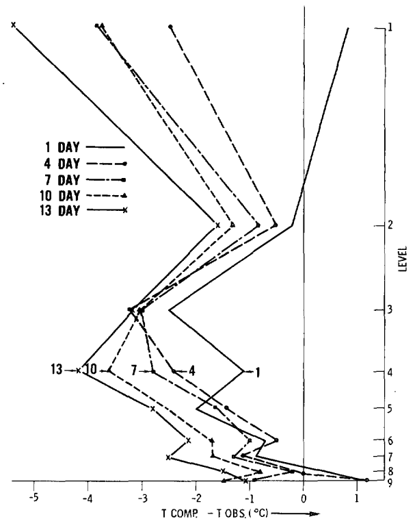
FIGURE 15.—Hemispherically averaged temperature error for Experiment 3 at 1, 4, 7, 10, and 13 days. The ordinate is the vertical level.
