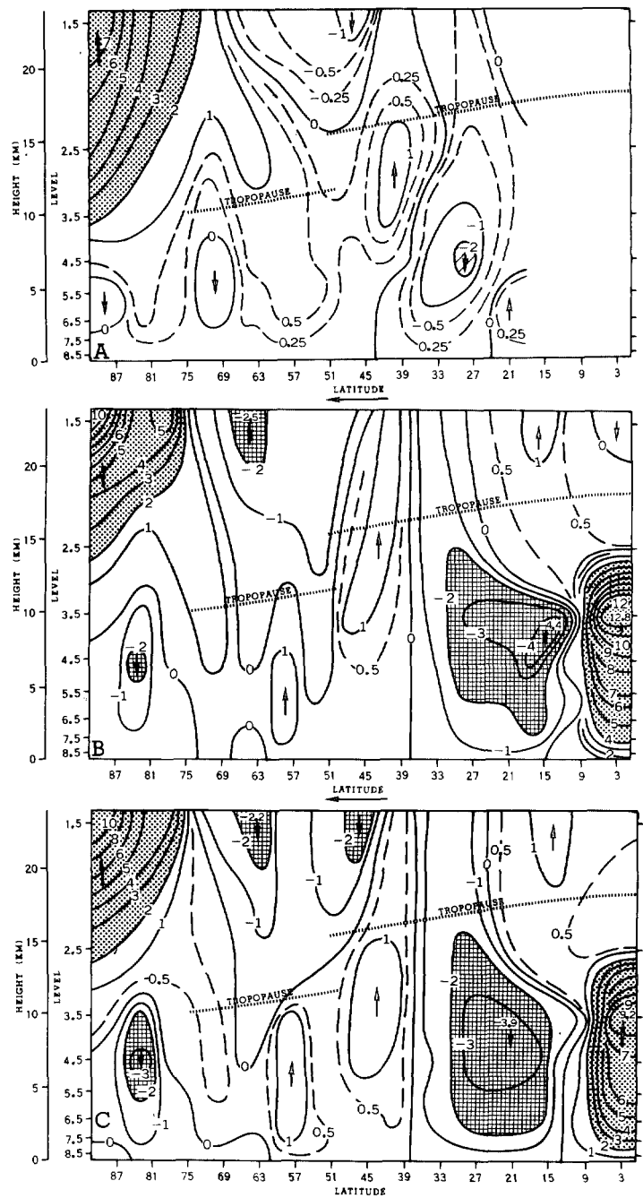
FIGURE 38.—Meridional section of the vertical velocity \overline{W} = \overline{dz/dt} in units of 10^{-1} cm/sec. The direction of velocity is indicated by arrows. The regions where the upward velocity is larger than 0.2 cm/sec are hatched, and the regions where the downward velocity is larger than 0.2 cm/sec are stippled. (A) computed by applying the \omega -equation to the data for each of the 14 days and then averaged, (B) Experiment 2, and (C) Experiment 3. The latter two are averaged for 3 to 14 days.
