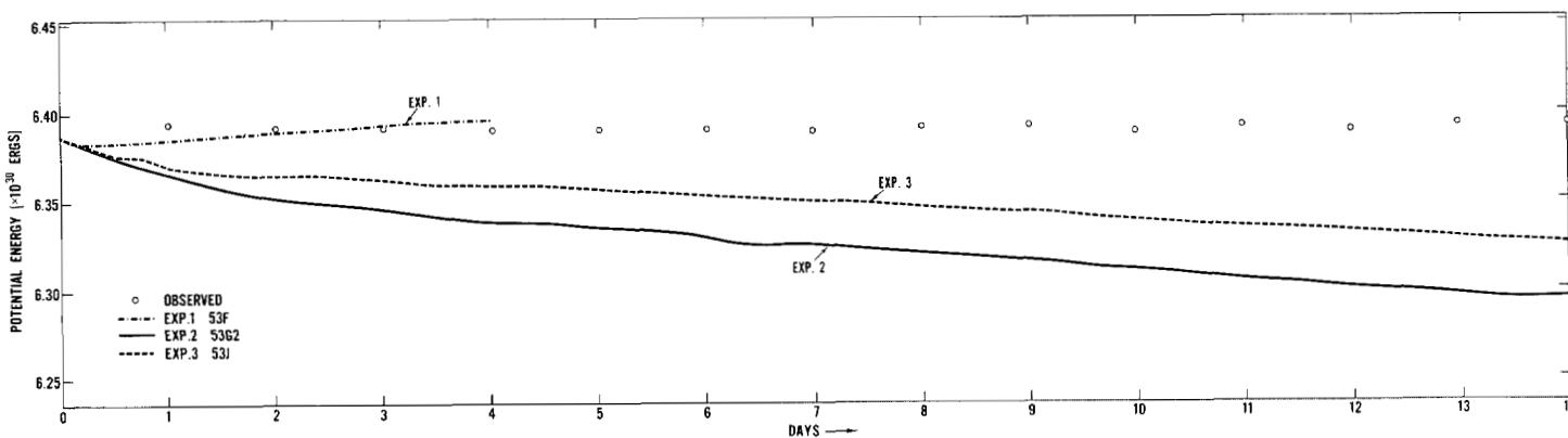
FIGURE 29.—Time variation of the internal plus potential energy integrated over the whole hemisphere for Experiments 1, 2, and 3 in units of 10^{30} ergs. The observed values are shown by small open circles.
