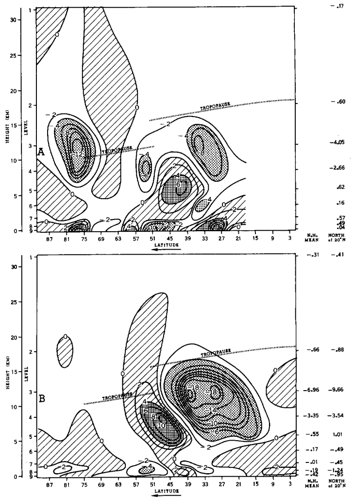
FIGURE 86.—Conversion from zonal kinetic to eddy kinetic energy \langle k_z \cdot k_E \rangle in units of 10^{-4} \text{ ergs cm}^{-3} \text{ sec}^{-1} . (A) observed data and from the \omega -equation, and (B) the prediction. See figure 65.
