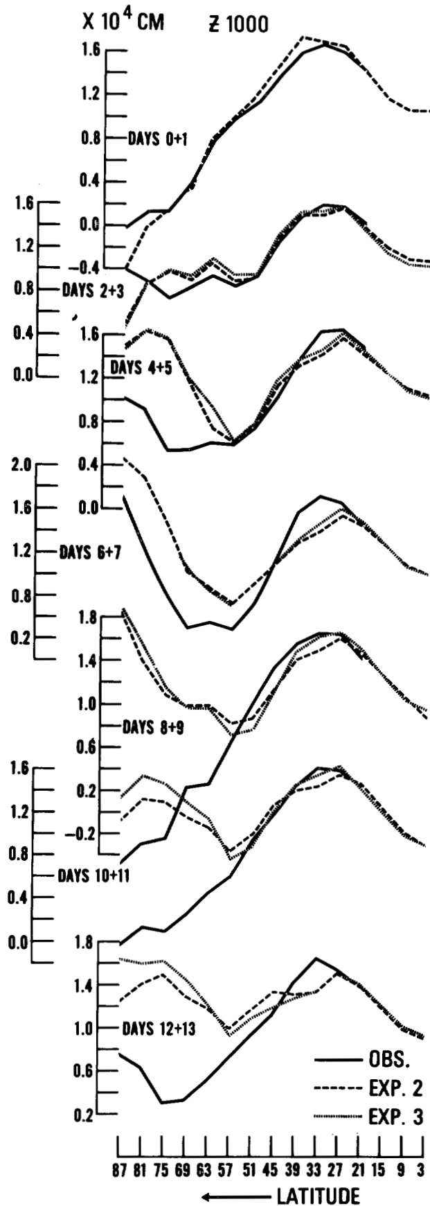
FIGURE 52.—Latitudinal distribution of 1000-mb geopotential height for the observed (solid lines), Experiment 2 and Experiment 3 for the 1964 case. Zonal averages and 2-day averages were taken. The computed results deviated largely from the observation especially at high latitudes.
