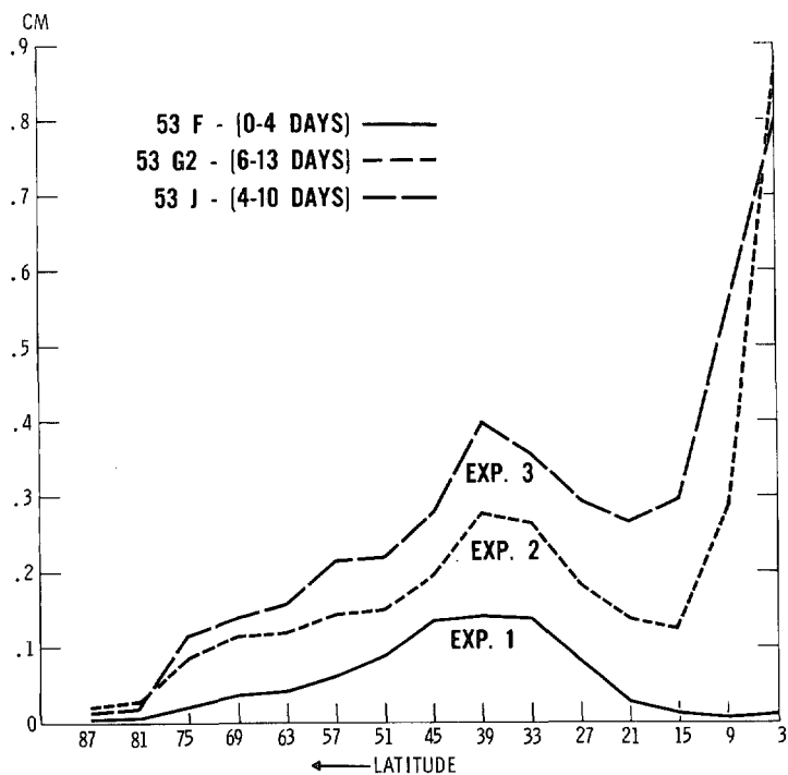
FIGURE 5.—Latitudinal distribution of the 24-hr rate of precipitation for Experiments 1, 2, and 3.
