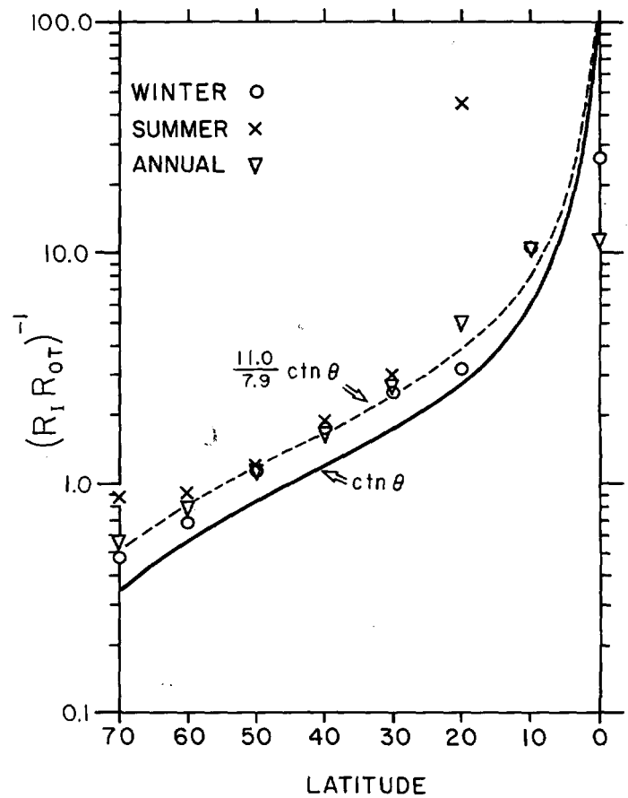
Figure B5.—A comparison of the theoretical equilibrium (R_I R_{OT})^{-1} and the observed (with \Theta_{PE} used instead of \Theta ).
