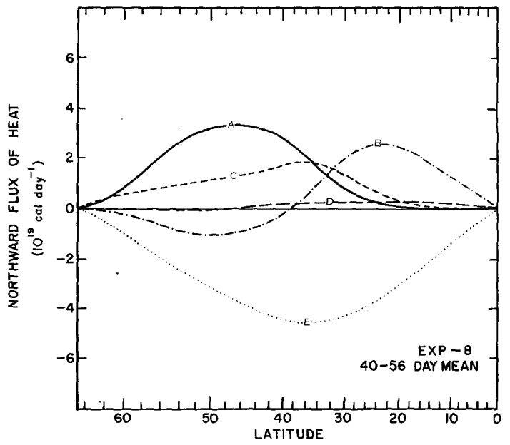
FIGURE 9.8.—Same as figure 9.7, but for the 40–56 day mean.
