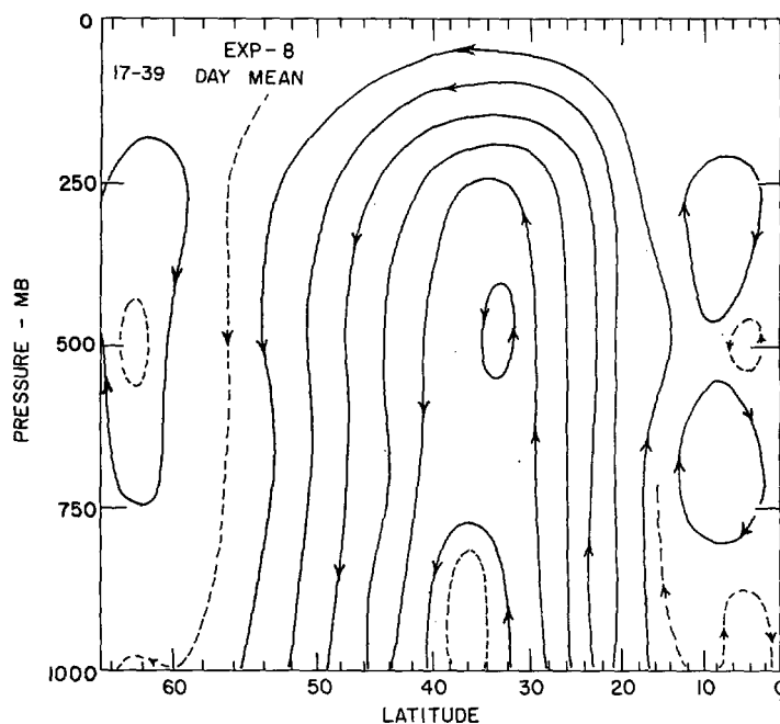
FIGURE 10.7.—The “streamlines” of the zonal angular momentum flux corresponding to the resultants in figure 10.6.
