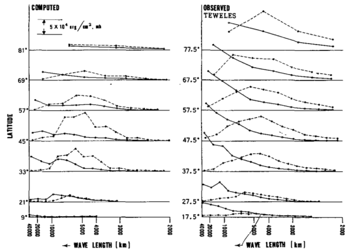
FIGURE 4D3.—The latitudinal variation of the effective wave number and of the meridional wind component are shown by solid and dashed lines, respectively.
