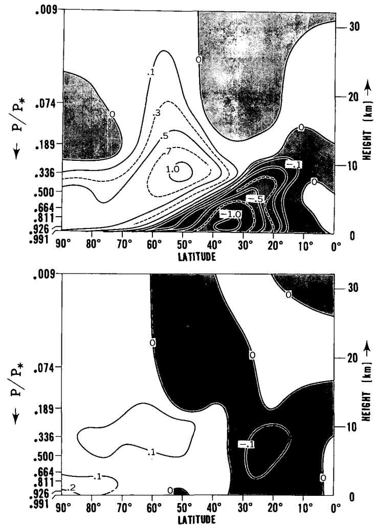
FIGURE 5D5.—The latitude-height distributions of the rate of temperature change ( ^{\circ}\text{C}/\text{day} ) due to large-scale eddies and subgrid-scale mixing are shown in the upper and lower parts of the figure, respectively.
