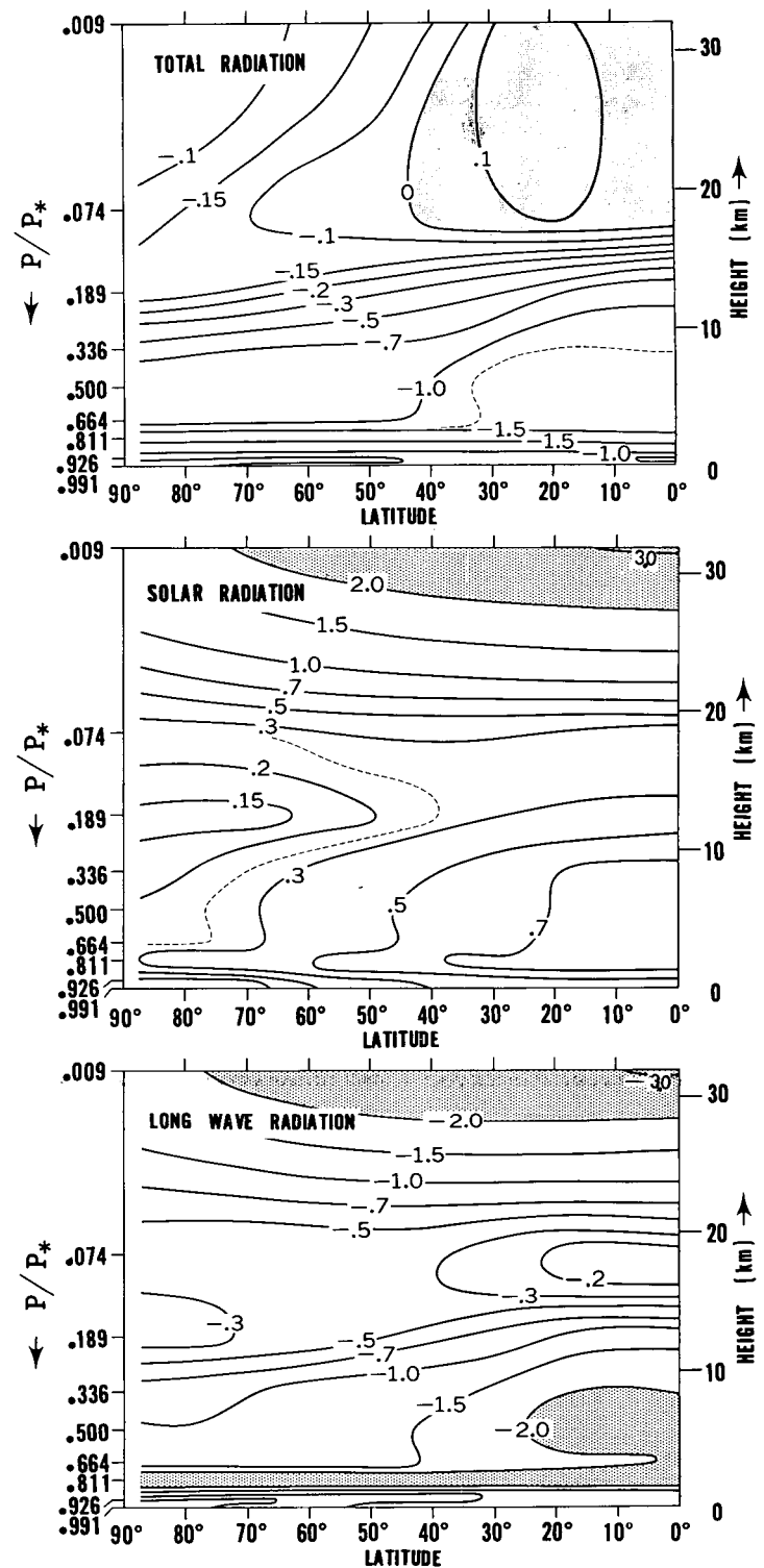
FIGURE 5D1.—Upper, middle, and lower parts of the figure give the latitude-height distributions of calculated temperature change ( ^{\circ}\text{C}/\text{day} ) due to the net rate of radiation, the solar radiation only, and long-wave radiation only.
