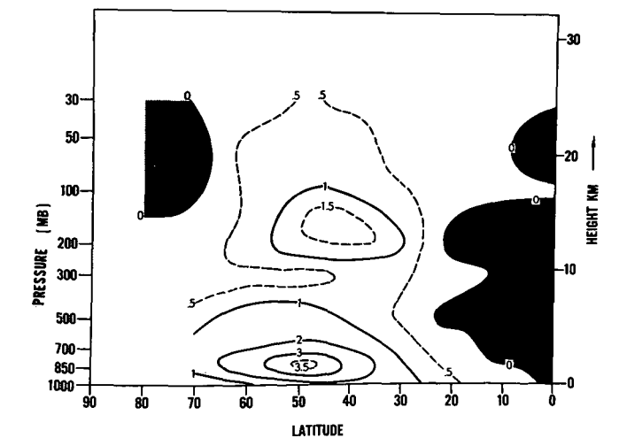
FIGURE 5D3.—The upper part of the figure shows the latitude-height distribution of the calculated poleward eddy transport of heat on isobaric surfaces. In the lower part of the figure the northward heat transport obtained by Starr and White [39] for the year 1950 is shown. Units are 10^{17} joule \text{mb.}^{-1} day. ^{-1}
