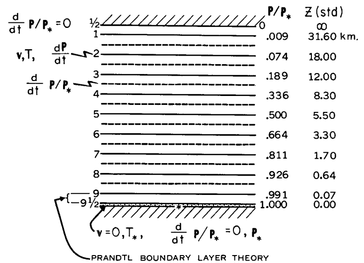
FIGURE 2F2.—Diagram of Q levels and their approximate heights. Notations are made as to where the model variables are predicted.
