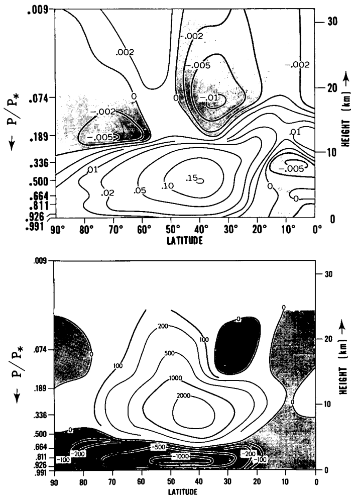
FIGURE 7C4.—The latitude-height distributions of -\overline{\omega' \alpha'}^H (in units of joule cm. -2 mb. -1 day -1 ) and that of -\overline{\omega' \phi'}^H (in units of 10 -2 joule cm. -2 day -1 ) on the isobaric surface are shown in the upper and lower parts of the figure, respectively.
