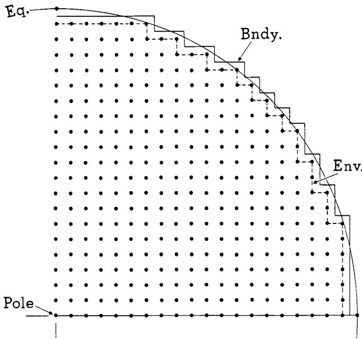
FIGURE 2F1.—Map of the grid points on which the computations were performed showing one quarter of the stereographic projection plane of the Northern Hemisphere ( N=20 ). The free-slip, insulated boundary (Bndy.) is located one-half-grid-point distance outside the envelope (Env.) of the southernmost grid points in the Northern Hemisphere, not including the four points on the Equator (Eq.) at the intersections of the coordinate axes.
