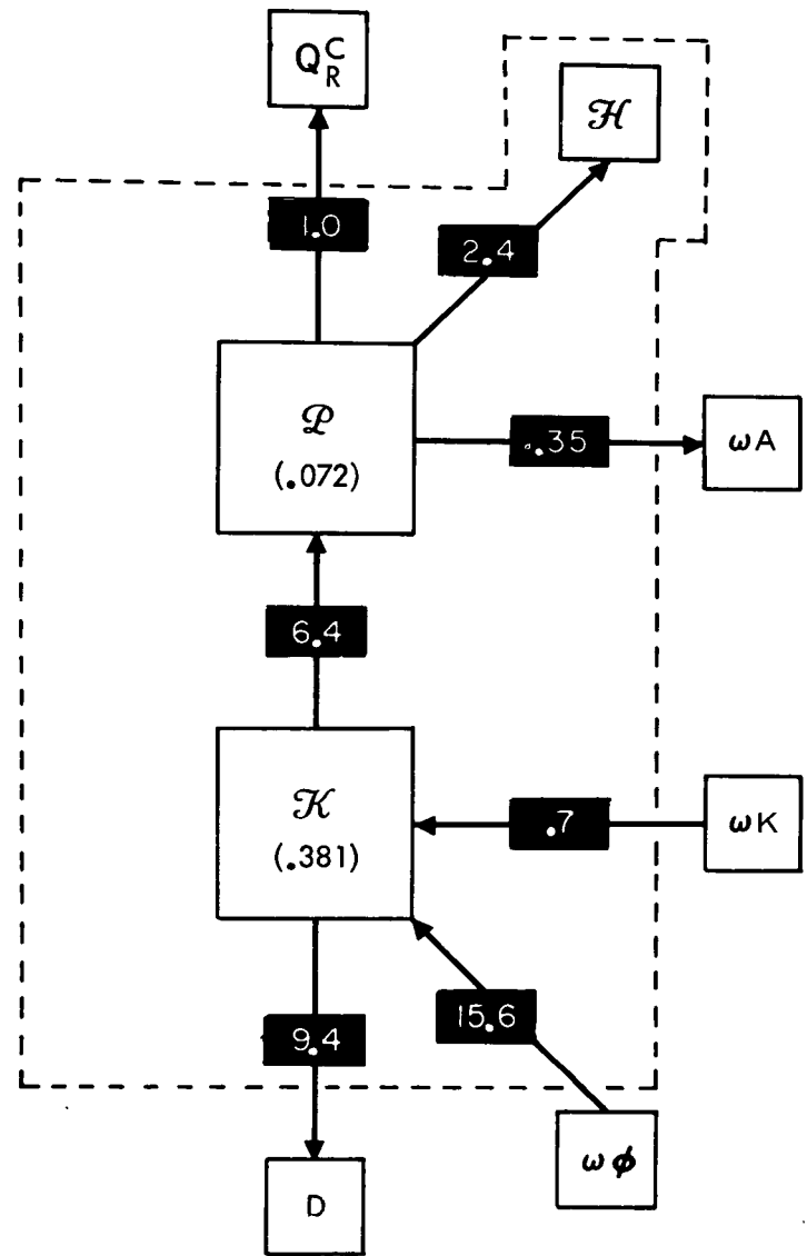
FIGURE 7F1.—Two-box energy diagrams for the model stratosphere (approximately the 34–126-mb. layer). Q_C^R , generation of available potential energy due to radiation and convection from the earth's surface. \omega A , the effect of the vertical transport of available potential energy. \omega K , the effect of vertical transport of kinetic energy. \omega \phi , effect of the pressure interaction term. The unit of energy transformation is 10^{-3} joule \text{mb.}^{-1} \text{cm.}^{-2} \text{day}^{-1} and the unit of energy itself is joule \text{cm.}^{-2} \text{mb.}^{-1} . For further explanation refer to figure 7A1. NOTE: Value of P_z should be .064 instead of .072.
