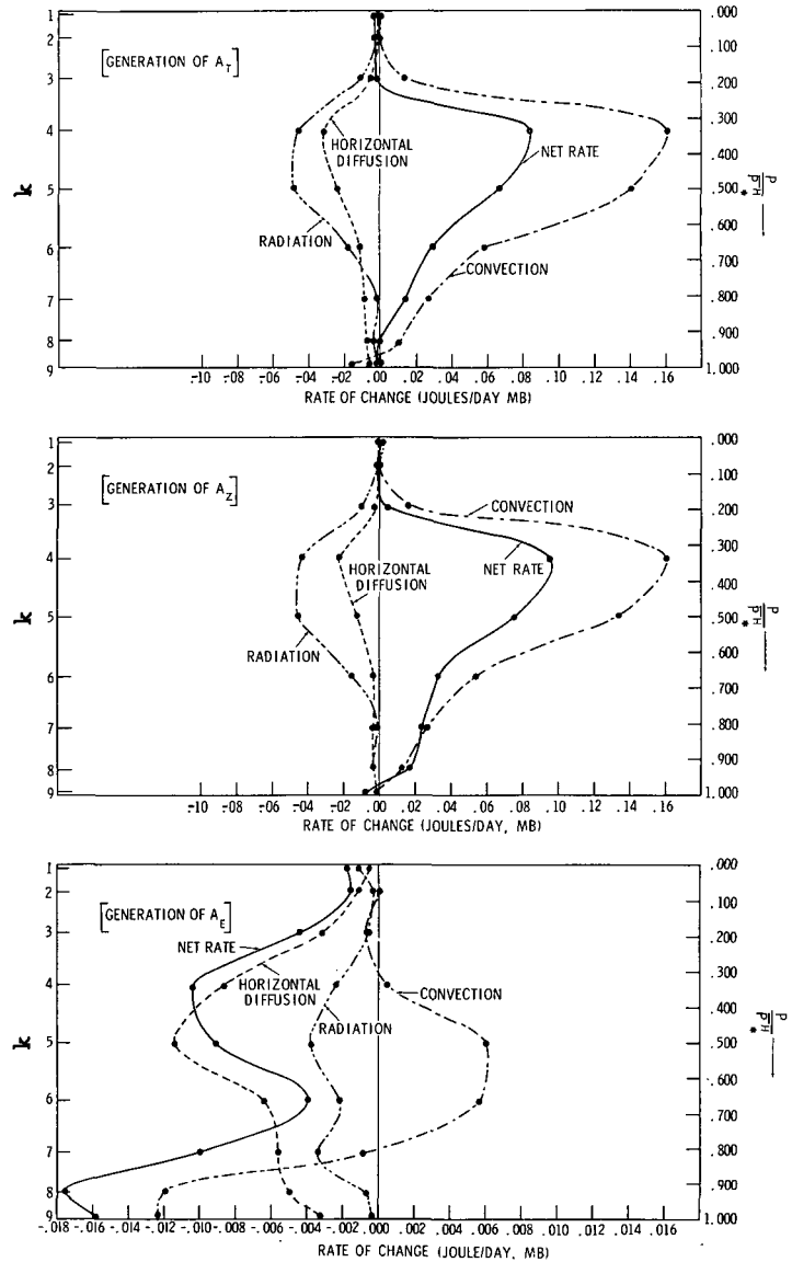
FIGURE 7D2.—The vertical distribution of the generation or destruction of available potential energy due to convection, radiation, and horizontal subgrid-scale mixing. The distributions for the total available potential energy, zonal available potential energy, and eddy available potential energy are shown in the upper, middle, and lower parts of the figure, respectively. Note the change of horizontal scale on the eddy graph.
