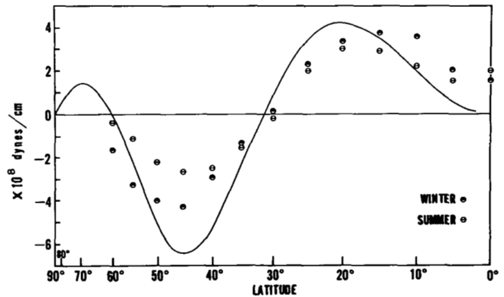
FIGURE 6A2.—The rates of the change of angular momentum due to meridional circulation, large-scale eddies, subgrid-scale diffusion, and surface torque are shown as functions of latitude. In the lower part of this figure the distribution of computed surface torque (solid line) is contrasted with the estimate of surface torque by Priestley [31] for the actual atmosphere (coded circles). The Priestley data are means for two hemispheres averaged by seasons.
