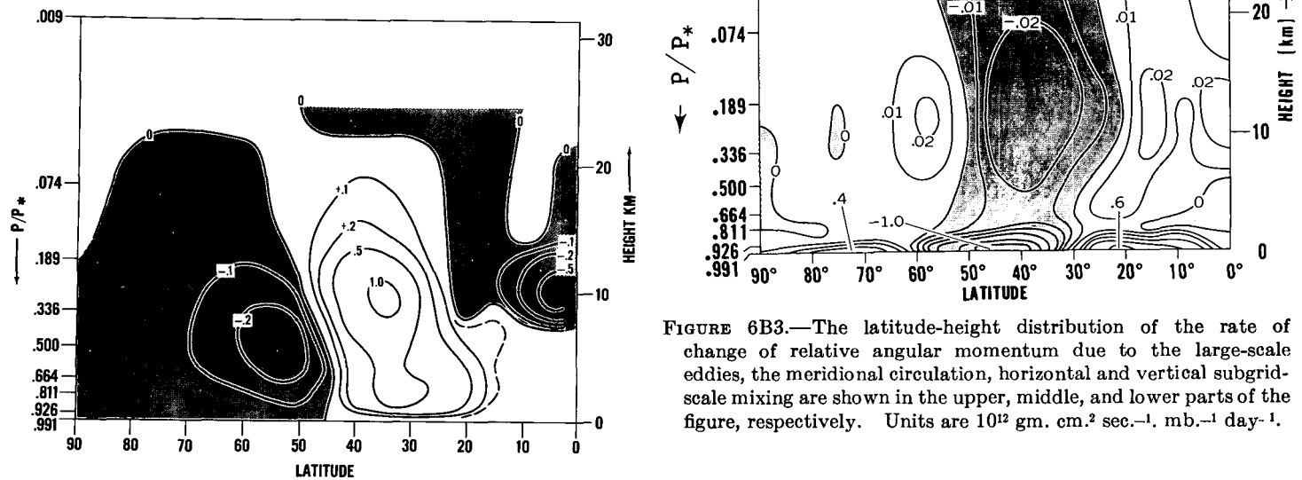
FIGURE 6B2.—Latitude-height distribution of vertical transport of angular momentum by the large-scale eddies. Unit is 10^{18} gm. sec. -1 day. -1
