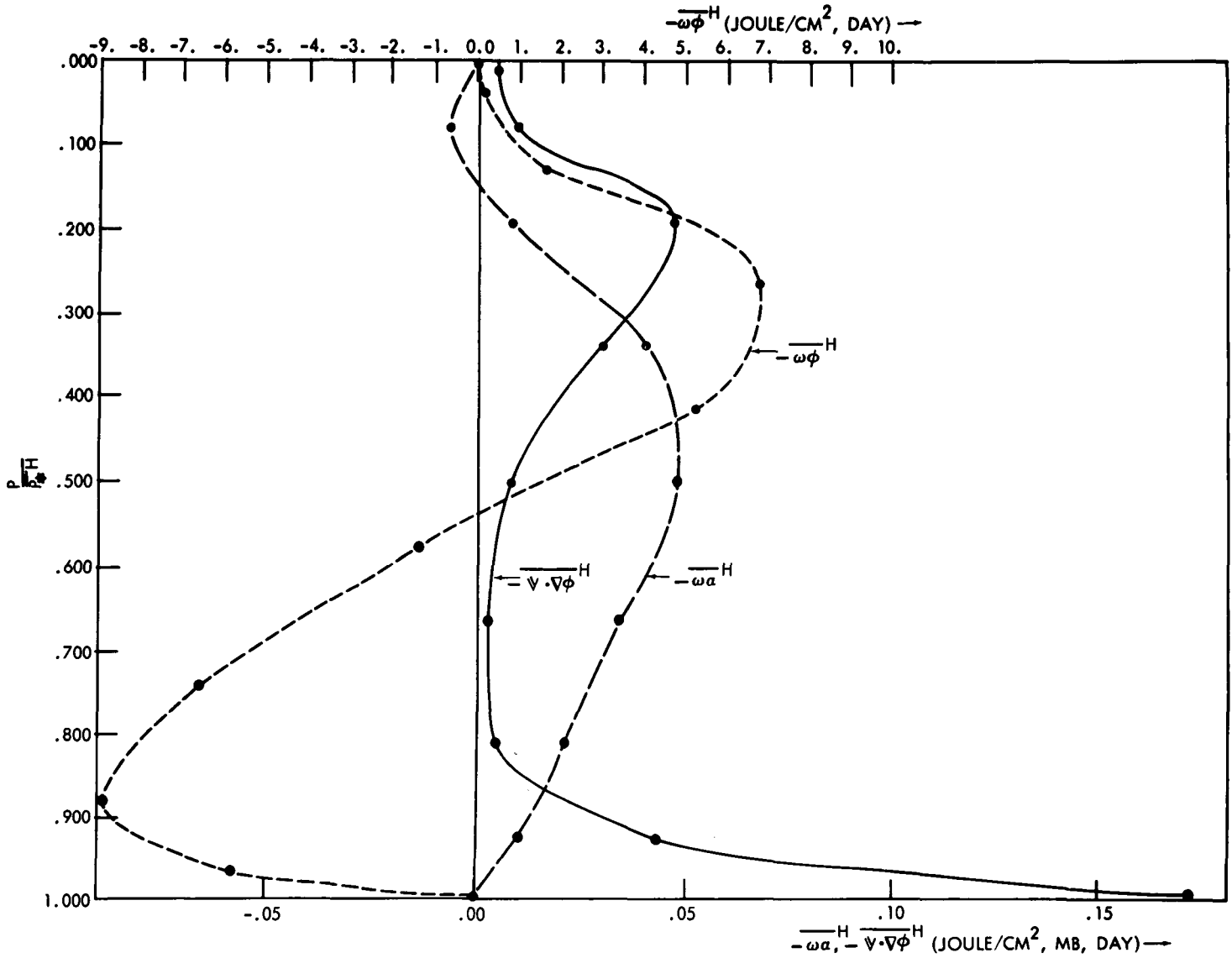
FIGURE 7B2.—Vertical distribution of -\overline{\nabla\cdot\nabla\phi}^H , -\overline{\omega\phi}^H , and -\overline{\omega\alpha}^H on an isobaric surface.
