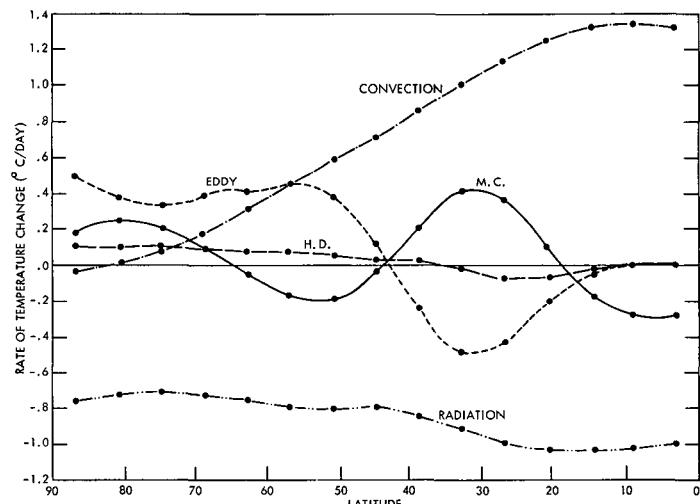
FIGURE 5B3.—The latitudinal distribution of temperature change due to convection, radiation, meridional circulation (M.C.), large-scale eddies (EDDY), and horizontal subgrid-scale mixing (H.D.) are shown.
