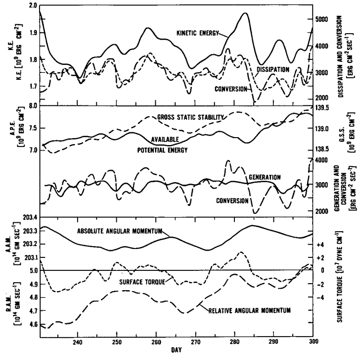
FIGURE 3.2.—In the upper part of the figure, the solid line shows the time variation of the hemispheric mean of kinetic energy for the period of 231-300 days, and the long-dashed and short-dashed lines show the time variation of the hemispheric mean of conversion and of dissipation, respectively. In the middle part of the figure, the time variation of total available potential energy and gross static stability are shown by solid and dashed lines respectively. The rate of generation (source) and conversion of available potential energy are also shown by solid and dashed lines respectively. In the lower part of the figure, the solid line and long-dashed line show the time series of the hemispheric mean of absolute angular momentum and of relative angular momentum for the period of 231-300 days, respectively. The short-dashed line shows the time variation of the hemispheric mean of surface torque.
