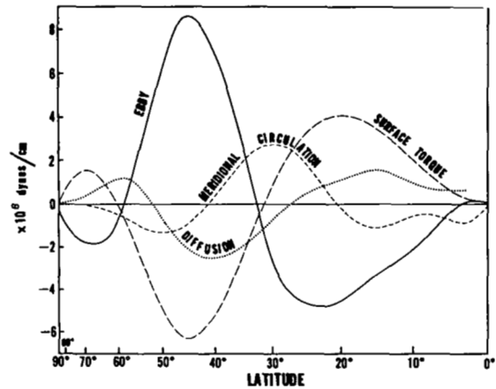
FIGURE 6A1.—The latitudinal distribution of northward transport of angular momentum due to various components. The transports due to meridional circulation, large-scale eddies, horizontal subgrid-scale mixing are shown by dotted, solid, and dashed lines, respectively. The annual mean values of momentum flux obtained by Starr and White [39] and those obtained by Buch [4] are plotted by stars and squares, respectively.
