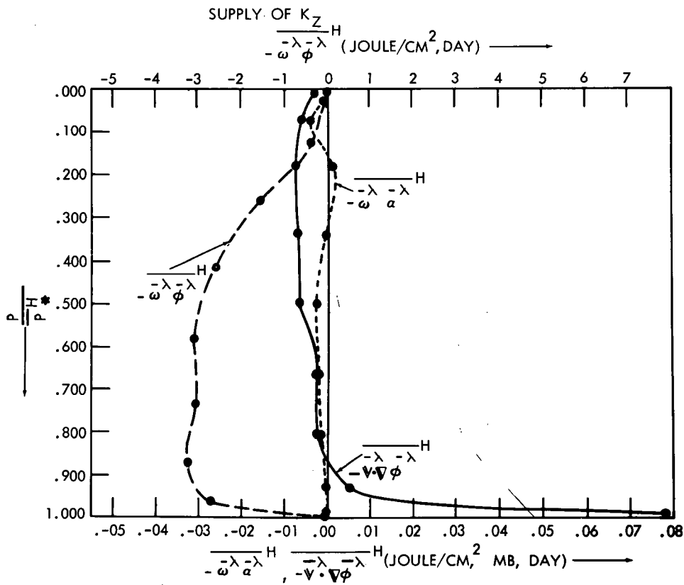
FIGURE 7C2.—The vertical distributions of -\overline{v \cdot \nabla \phi'^H} , -\overline{w'a'^H} , and -\overline{w'\phi'^H} are shown in the upper part of the figure and those of -\overline{v \cdot \nabla \phi^H} , -\overline{\omega \lambda \phi^H} , and -\overline{\omega \lambda \phi \lambda^H} are shown in the lower part of the figure. These terms are on isobaric surfaces.
