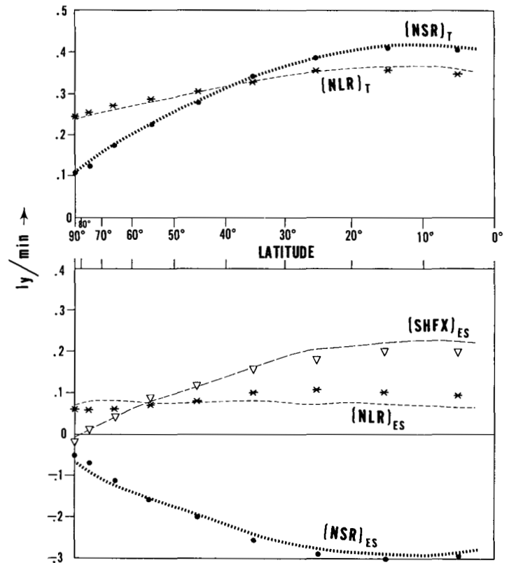
FIGURE 5B1.—The upper half of the figure shows curves of the latitudinal distribution of net upward long-wave radiation (NLR)_T and that of net downward solar radiation (NSR)_T at the top of the atmosphere. The lower half of the figure shows the latitudinal distribution of the net upward long-wave radiation (NLR)_{ES} , of net upward solar radiation (NSR)_{ES} , and of the upward turbulent flow of heat (SHFX)_{ES} at the earth's surface. The corresponding quantities obtained by London [14] are plotted in the same figure as stars, dots, and triangles for comparison.
